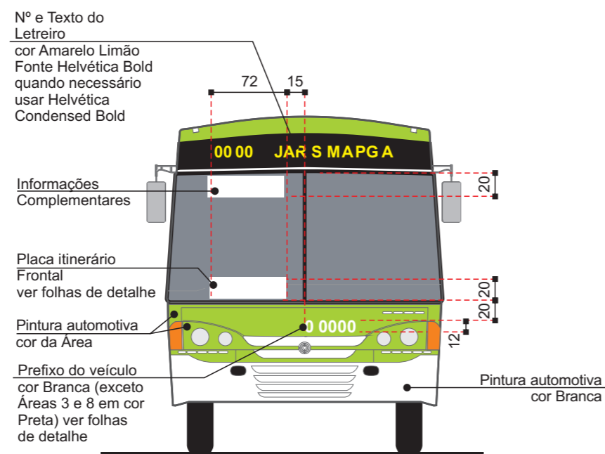
Vista frontal
