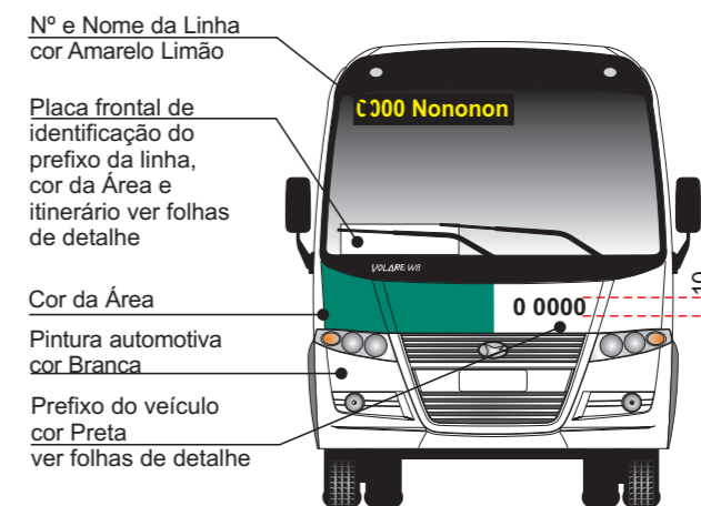
Vista frontal
