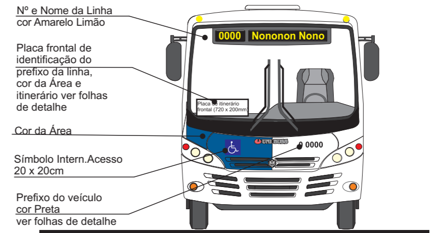
Vista frontal
